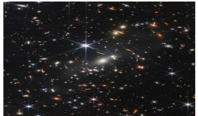
(The farthest cosmos pictured by telescope)
